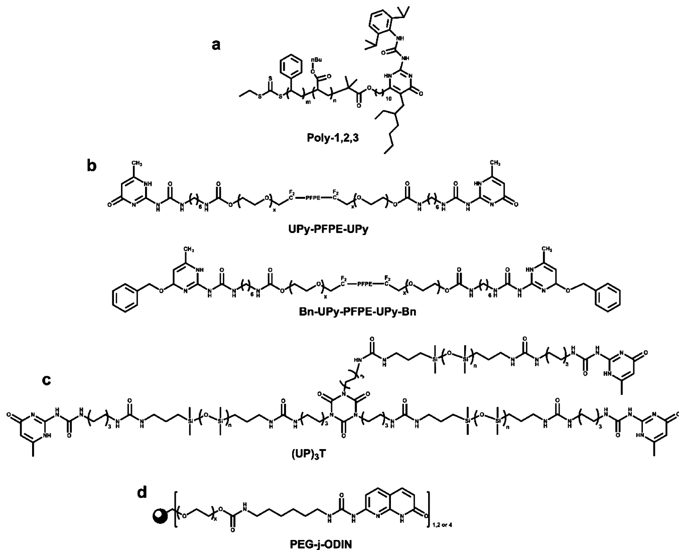
Figure 6. Chemical structures of self-healing elastomers with hydrogen-bonding units as chain ends (a–d).
