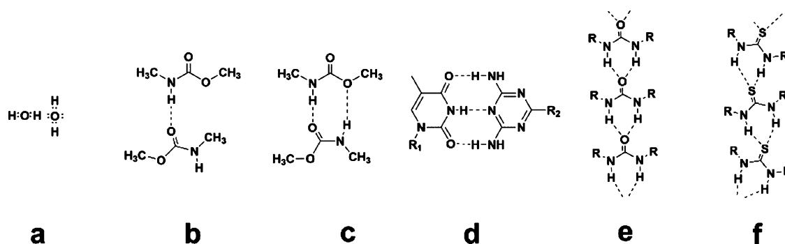
Figure 3. Chemical structures of hydrogen bonding in water molecules (a), single (b), double (c), triple (d), linear array (e), and zigzag array (f) of hydrogen bonding.
