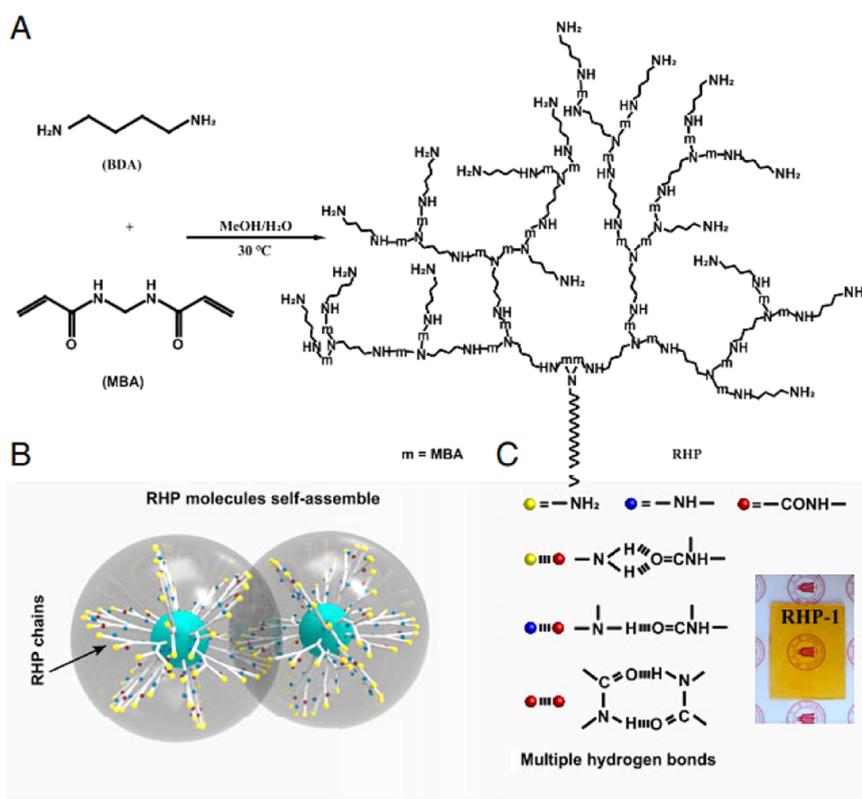
Figure 9. Design concept and synthesis of RHP. (A) Chemical route to the synthesis of RHP through Michael addition between MBA and BDA at 30 °C. (B) Schematic diagram of interactions between RHP molecules. (C) Multiple hydrogen bonds of RHP molecules. (Inset) A photograph of RHP-1. 65 Reproduced with permission. Copyright (2020) National Academy of Sciences.
