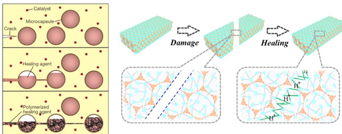
Figure 1. Extrinsic (left) and intrinsic self-healing process. 14,15 (left) Reproduced with permission. Copyright (2001) Springer Nature. (right) Reproduced with permission. Copyright (2017) National Academy of Sciences.
