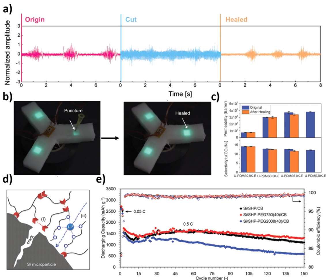
Figure 17. (a) Ambulatory EMG monitoring when the DAE electrode was cut off and after healing. 78 (b) Photographs showing the HELIOS device healed immediately after a puncture. 79 (c) Comparative gas-separation performance of original polymer membranes (blue) and polymer membranes after being cut and healing (orange), CO 2 permeability (up), and CO 2 /N 2 selectivity (bottom). 80 (d) Self-healing polymeric (SHP-PEG) binder enabled by multiple H-bond interactions for maintaining the integrity of the Si electrodes during charge–discharge cycles. (e) Cycle performances and coulombic efficiency of the Si electrode with a varied SHP-PEG binder. 81 (a) Reproduced with permission from ref 78. Copyright 2018, Wiley-VCH. (b) Reproduced with permission from ref 79. Copyright 2020 Springer Nature. (c–e) Reproduced with permission from ref 80. Copyright 2018, Wiley-VCH.
