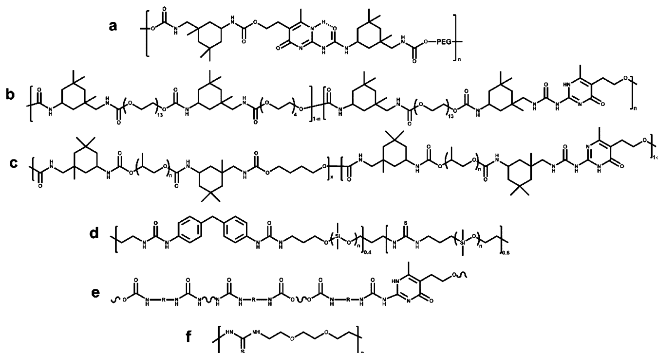
Figure 7. Chemical structures of self-healing elastomers with hydrogen-bonding units in the mainchain (a–f).
