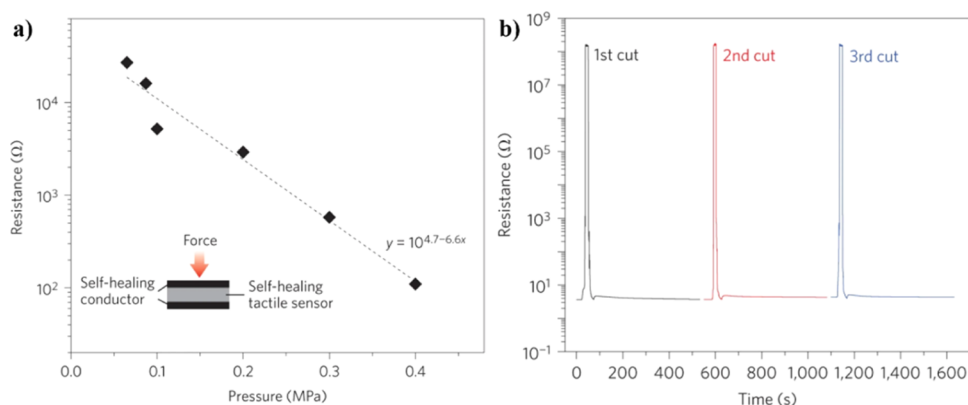
Figure 11. (a) Tactile sensor response at increasing peak pressure values (inset: sensor schematic). Equation represents least-squares fit relationship (dotted line) of resistance and applied pressure. (b) Repeated electrical healing for three cuts at the same severed location. 68 Reproduced with permission. Copyright (2012) Springer Nature.
