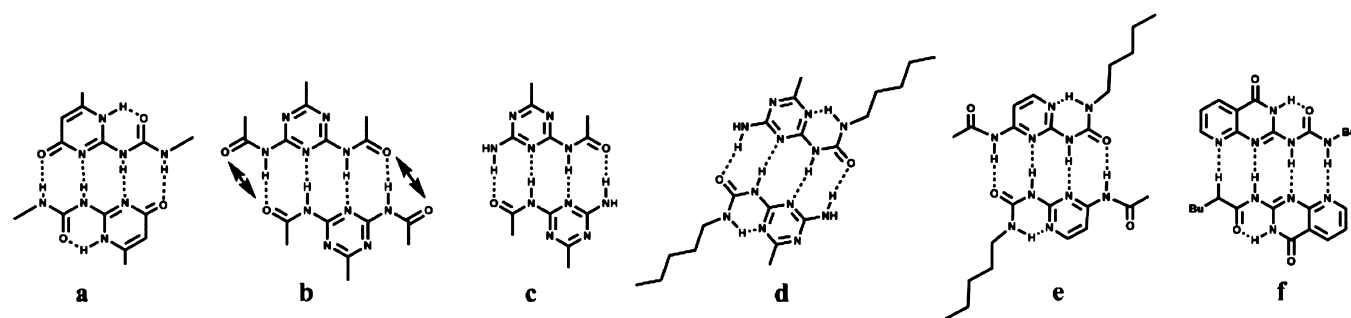
Figure 5. Several frequently used quadruple hydrogen-bonding units (a–f).
