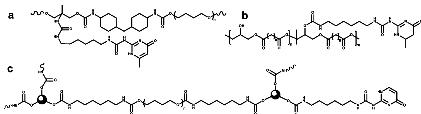
Figure 8. Chemical structures of self-healing elastomers with hydrogen-bonding units in the sidechain (a–c).
