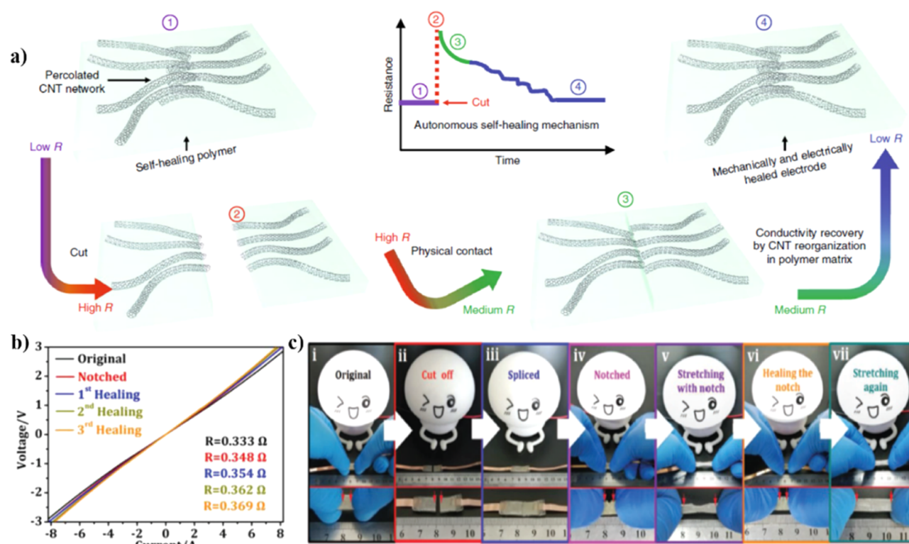
Figure 10. (a) Proposed recovery mechanism for CNTs embedded in a self-healing polymer matrix. 66 (b) I – V curves of the conductive film after several cutting–healing cycles. (c) Demonstration of electric conductivity retention capability under various situations (i) original, (ii) cut, (iii) after healing, (iv) healed specimen with a notch, (v) healed specimen with a notch was stretched to 300% strain, (vi) stretched specimen with a notch was unloaded and then rested for 12 h, (vii) when the specimen was stretched to 300% strain again, the conductivity remained. Surprisingly, the notch vanished. 67 (a) Reproduced with permission. Copyright (2018) Springer Nature. (b,c) Reproduced with permission. Copyright (2020) Wiley-VCH.
