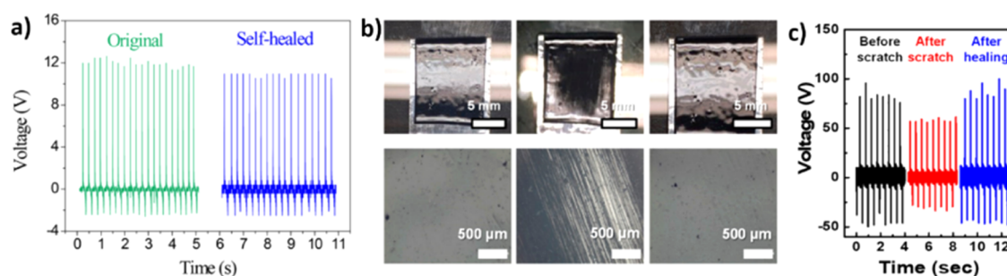
Figure 14. (a) Output voltage (VOC) of s-TENG after self-healing at ambient for 72 h. 72 (b) Digital photographs (top) and optical images (bottom) of polymer composites with 0.2 wt % o-CNT before and after healing at 90 °C and 80% humidity condition. (c). Triboelectric output voltage of the self-healable polymer composite with 0.2 wt % o-CNT before and after healing. 73 Copyright (2020) ACS.
