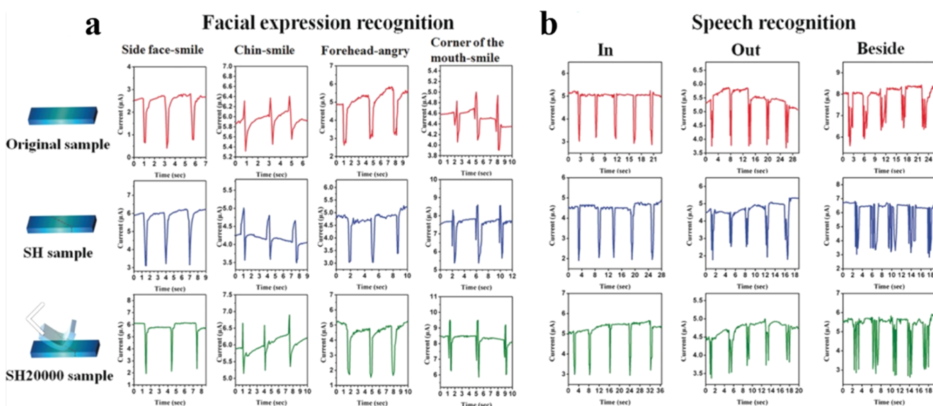
Figure 12. Current responses of the original, self-healed (SH), and SH20000 strain sensors in (a) facial expression recognition at different facial parts and (b) vocal-cord vibrations with the tester pronouncing different words. SH sample and SH sample after bending over 20,000 times (SH20000). 25 Reproduced with permission. Copyright (2017) Wiley-VCH.
