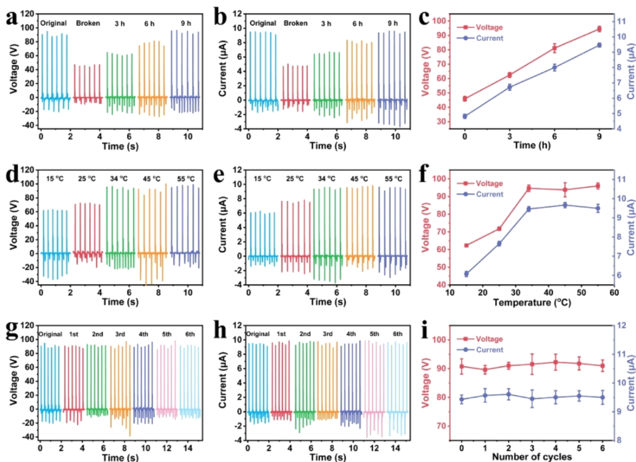
Figure 15. Output characteristics of IU-TENG under varying healing conditions. (a) Open-circuit voltage and (b) short-circuit current of the original, broken, and SH IU-TENG after three different healing times from 3 to 6 h and then to 9 h at 34 °C. (c) Voltage and current changes of IU-TENG after different healing times at 34 °C. (d) Open-circuit voltage and (e) short-circuit current of SH IU-TENG at different temperatures (15, 25, 34, 45, and 55 °C) for 9 h. (f) Voltage and current changes of IU-TENG at different healing temperatures for 9 h. (g) Open-circuit voltage and (h) short-circuit voltage of the original and SH IU-TENG after one to four cycles under NIR irradiation. (i) Voltage and current changes of IU-TENG after healing under NIR irradiation for several cycles (0 represent the original). 74 Reproduced with permission from ref 74. Copyright (2020) Wiley-VCH.
