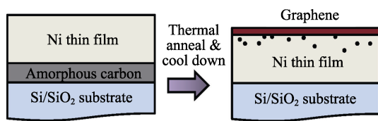
图 3 热退火方法金属催化非晶碳转化石墨烯示意图 [31] Fig. 3 Process schematic for the metal-catalyzed crystallization of a-C to graphene by thermal annealing [31]
