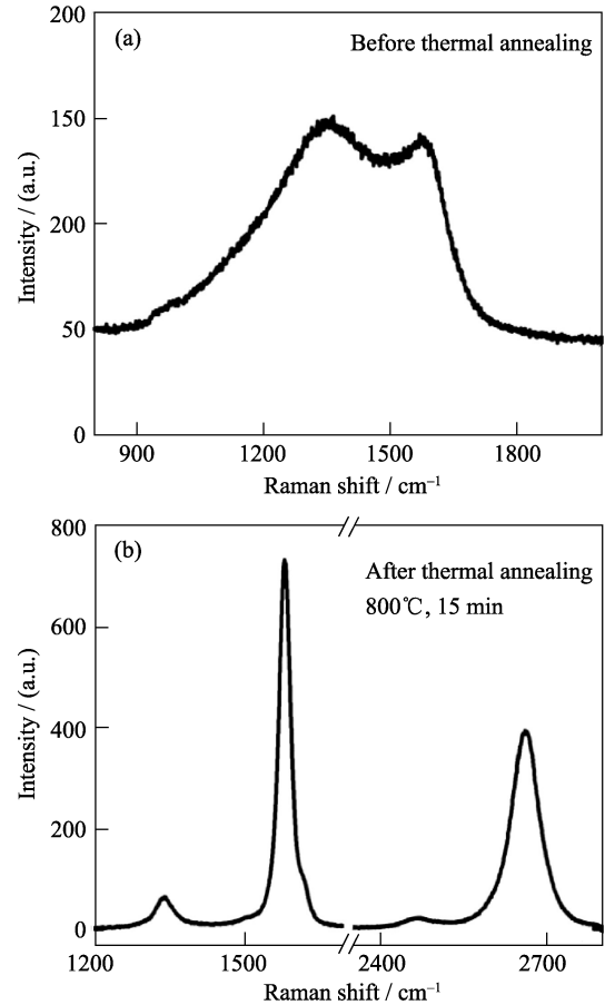
图 5 (a) a-C(40 nm)和(b)Ni 催化结晶后得到的石墨烯(Ni 厚度~300 nm)的 Raman 光谱图, 激光发射波长 632.8 nm [31] Fig. 5 Raman spectra of (a) a-C (40 nm) and (b) the resulting graphene layer after Ni-catalyzed crystallization (Ni thickness ~300 nm) with excitation laser wavelength 632.8 nm [31]
