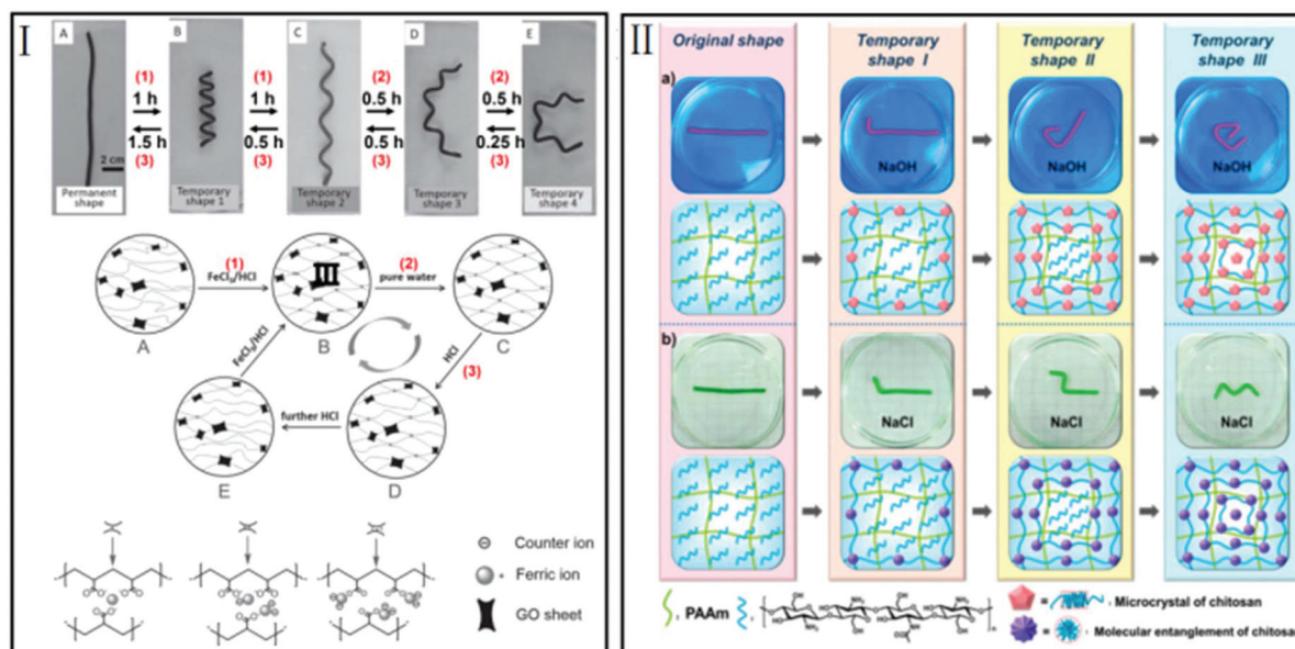
Fig. 5 Time-controlled multi-shape memory effect. (I) Adjusting the types of formation between Fe 3+ and AAC (mono-, bi-, and tridentate) by changing the immersing time in a FeCl 3 /HCl or HCl solution for multi-shape memory (reproduced from ref. 48 with permission of John Wiley and Sons); (II) different degrees of formation of microcrystals or molecular entanglement of chitosan for multi-shape memory (reproduced from ref. 49 with permission of MDPI).
